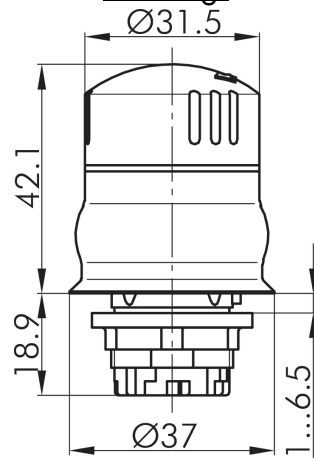
Dimensional drawing:
